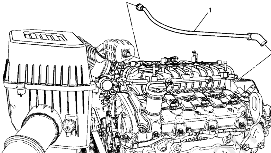
Fig. 19: Positive Crankcase Ventilation Tube - Front Courtesy of GENERAL MOTORS CORP.
