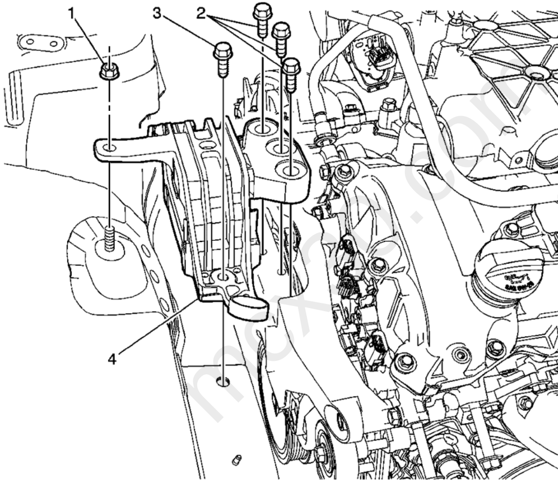
Fig. 16: Engine Mount - Right Side
