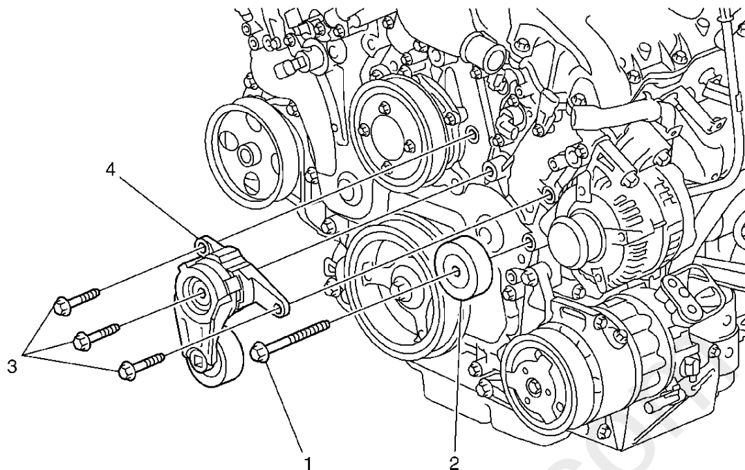
Fig. 2: Drive Belt Tensioner Courtesy of GENERAL MOTORS CORP.
