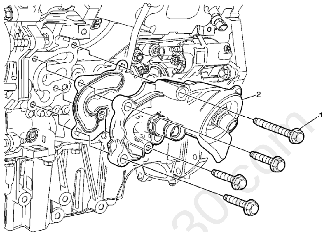
Fig. 34: Oil Filter Adapter Courtesy of GENERAL MOTORS CORP.
